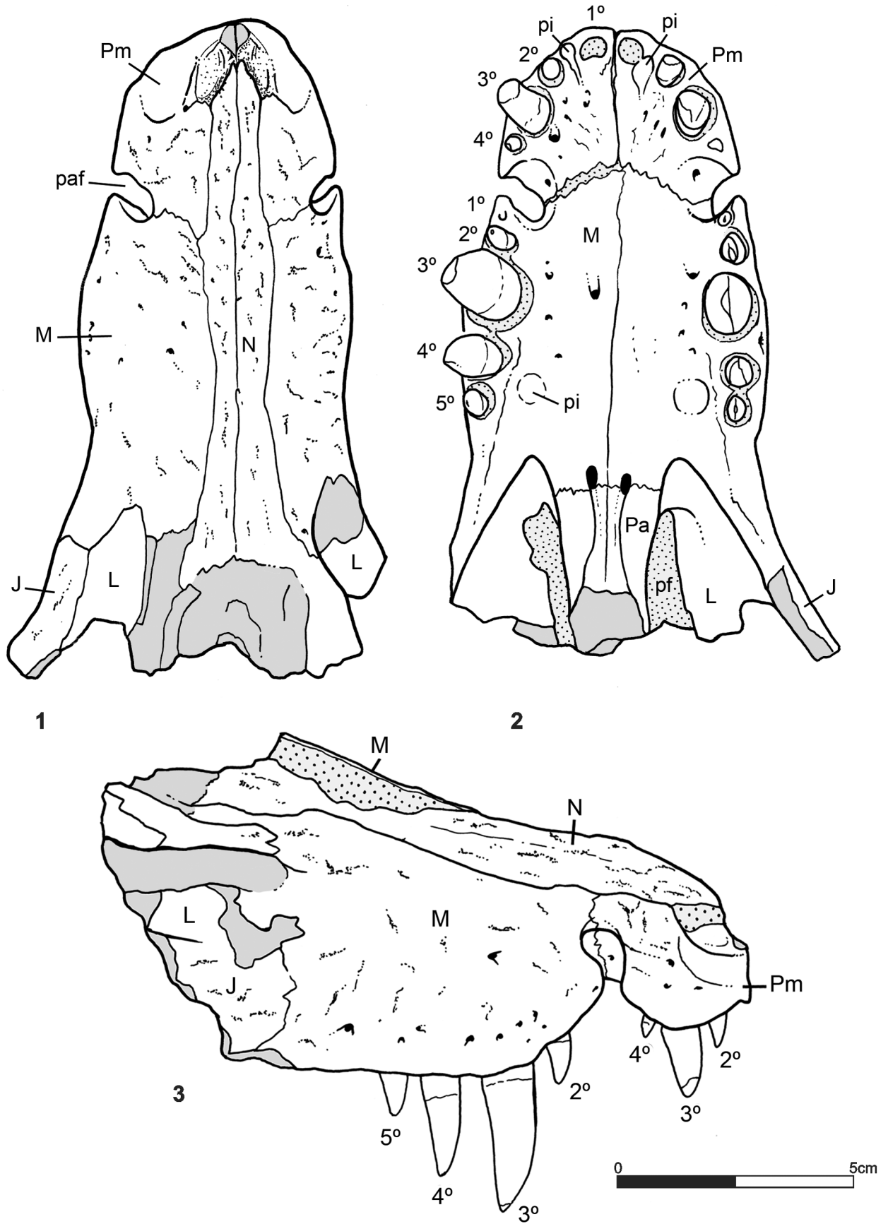
PLATE 6. Schematic drawings of specimen CPP 1236 of Campinasuchus dinizi gen. nov. et sp. nov. 1, dorsal view; 2, palatal view; and 3, right lateral view of the partial skull. Grey indicates broken surfaces and regular dotted grey indicates matrix.
