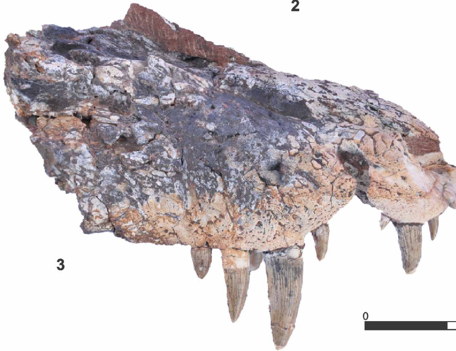
PLATE 5. Specimen CPP 1236 of Campinasuchus dinizi gen. nov. et sp. nov. 1, dorsal view; 2, palatal view; and 3, right lateral view of the partial skull.
